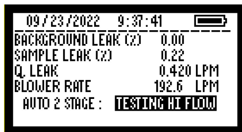
Figure 9. During the first stage, it will be display “Testing Hi Flow” for 90 seconds, this is followed by 90 seconds in the low flow or second stage which is 70 – 80% of the Hi Flow/First Stage.
