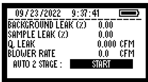
Figure 8. Prior to beginning the automatic – 2 stage test. The user must affix the end attachment on the leaking source and then press enter to start the test.
